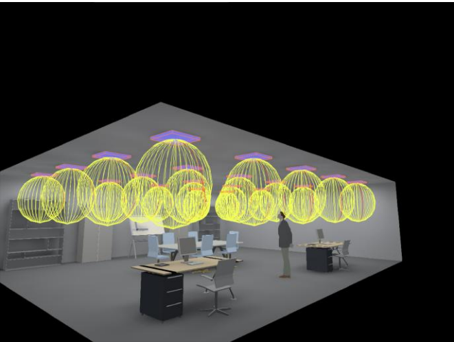
Office view with light distribution curves
