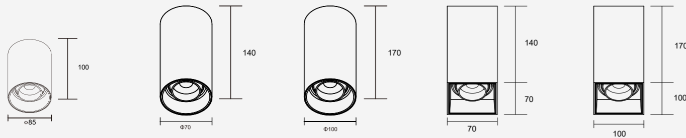
KS-MD16-A-415 Power:15W/20W Diameter:100mm Height: 170mm
