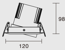
KAS-CL08R-4T Power: 15W/20W Cutout: 110mm Height: 98mm
