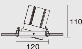
KAS-CL08R-4T Power: 30W Cutout: 110mm Height: 110mm
