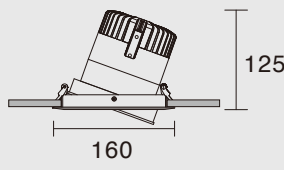
KAS-CL08R-5T Power: 30W/40W Cutout: 145mm Height: 125mm
