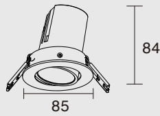
KAS-CL08R-3T Power: 10W Cutout: 75mm Height: 84mm
