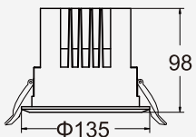
KS-CL39R-1V-525F-2 Power: 25W Cutout: 125mm Height: 98mm
