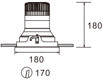
KAS-CL13R-6F Power:30W/40W Cutout: 170mm Height: 180m
