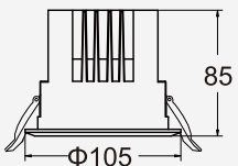
KS-CL39R-1V-420F-2 Power: 20W Cutout: 95mm Height: 85mm
