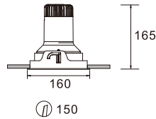
KAS-CL13R-5F Power:15W/20W/25W Cutout: 150mm Height: 165m
