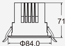
KS-CL39R-1V-315F-2 Power: 15W Cutout: 75mm Height: 71mm
