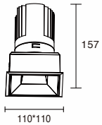
K-CL36-4F-S1D Power: 25W/30W Cutout: 100*100mm Height: 157mm
