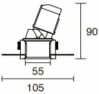
K-CL36-55T-R3D Power: 5W Cutout: 55mm Height: 90mm
