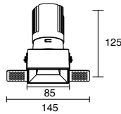
K-CL36-3F-S3D Power: 15W Cutout: 75*75mm Height: 125mm
