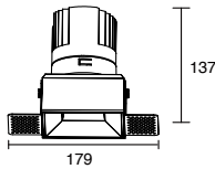
K-CL36-4F-S3D Power: 20W Cutout: 100*100mm Height: 137mm
