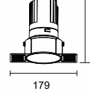
K-CL36-4F-R3D Power: 25W/30W Cutout: 100mm Height: 157mm
