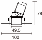
K-CL36-2T-R3D Power: 3W/5W Cutout: 55mm Height: 78mm
