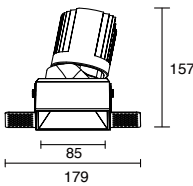
K-CL36-4T-S3D Power: 25W/30W Cutout: 100*100mm Height: 157mm
