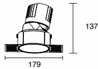
K-CL36-4T-R3D Power: 20W Cutout: 100mm Height: 137mm
