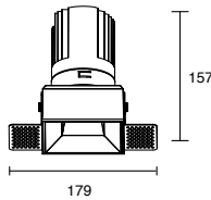
K-CL36-4F-S3D Power: 25W/30W Cutout: 100*100mm Height: 157mm
