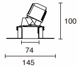
K-CL36-3T-R3D Power: 10W/12W Cutout: 83mm Height: 110mm
