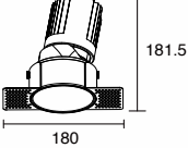
K-CL36-5T-R3D Power: 25W/30W Cutout: 123mm Height: 157mm
