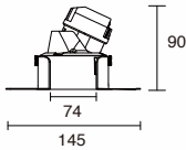
K-CL36-3T-R3D Power: 5W/8W Cutout: 83mm Height: 90mm
