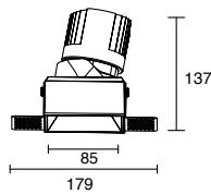
K-CL36-4T-S3D Power: 20W Cutout: 100*100mm Height: 137mm
