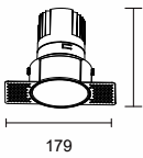
K-CL36-4F-R3D Power: 20W Cutout: 100mm Height: 137mm
