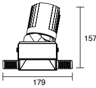
K-CL36-4T-S3D Power: 25W/30W Cutout: 100*100mm Height: 157mm
