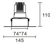
K-CL36-3F-S3D Power: 10W/12W Cutout: 75*75mm Height: 110mm
