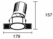
K-CL36-4T-R3D Power: 25W/30W Cutout: 100mm Height: 157mm
