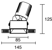
K-CL36-3T-S3D Power: 15W Cutout: 75*75mm Height: 125mm
