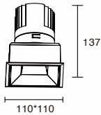
K-CL36-4F-S1D Power: 20W Cutout: 100*100mm Height: 137mm
