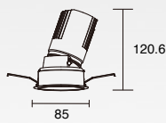
K-CL38-3T-R2D Power: 18W Cutout: 75mm Height: 120.6mm
