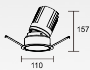
K-CL38-4T-R2D Power: 25W/30W Cutout: 90-95mm Height: 157mm
