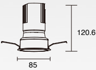
K-CL38-3F-R2D Power: 18W Cutout: 75mm Height: 120.6mm
