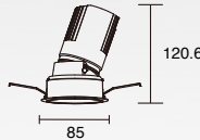
K-CL38-3T-R2D Power: 18W Cutout: 75mm Height: 120.6mm
