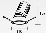
K-CL38-4T-R2D Power: 25W/30W Cutout: 90-95mm Height: 157mm
