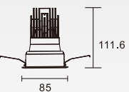
K-CL38-3F-R2D Power: 10W/12W/15W Cutout: 75mm Height: 111.6mm
