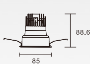
K-CL38-3F-R2D Power: 5W/8W Cutout: 75mm Height: 88.6mm
