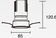
K-CL38-3F-R2D Power: 18W Cutout: 75mm Height: 120.6mm
