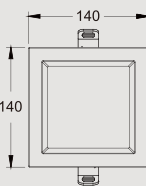
KAS-DL16-A-4 Power: 12W/15W Cutout: 125*125mm Height:38.3mm
