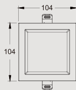
KAS-DL16-B-3 Power: 7W/9W/12W Cutout: 90*90mm Height:36.3mm
