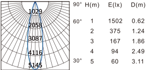
Beam angle:24° Luminous flux:1195lm
