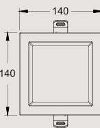
KAS-DL16-B-4 Power: 12W/15W Cutout: 125*125mm Height:38.3mm
