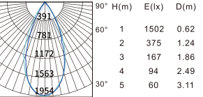
Beam angle:50° Luminous flux:1286lm
