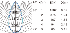
Beam angle:50° Luminous flux:980lm
