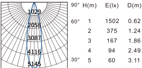
Beam angle:24° Luminous flux:915lm
