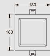
KAS-DL16-B-6 Power: 15W/20W/23W Cutout: 160*160mm Height:41.3mm
