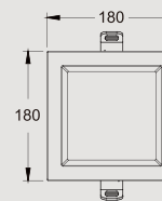
KAS-DL16-A-6 Power: 15W/20W/23W Cutout: 160*160mm Height:41.3mm
