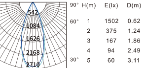
Beam angle:36° Luminous flux:929lm
