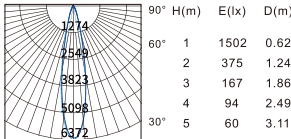
Beam angle:18° Luminous flux:818lm
