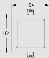
KAS-DL16-A-3 Power: 7W/9W/12W Cutout: 90*90mm Height:36.3mm
