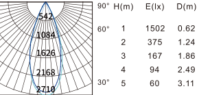
Beam angle:36° Luminous flux:1217lm
