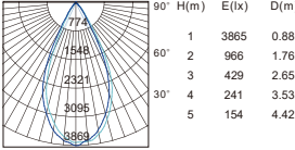
Beam angle 50° Luminous flux:2523lm
