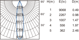
Beam angle 24° Luminous flux:2486lm
