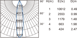
Beam angle 24° Luminous flux:2908lm
