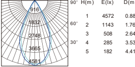
Beam angle 50° Luminous flux:2899lm
