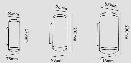
WL149-60-2x4W
