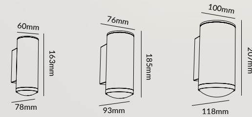
WL149-60-5W
